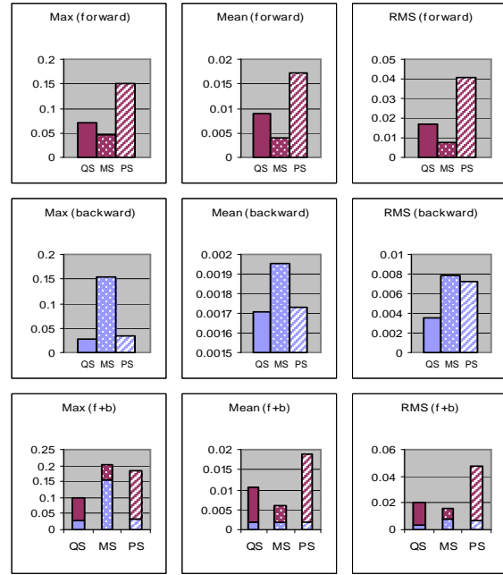
Figure 18: Max, mean, and RMS error values for the armoire model simplifications of 94 triangles (from lod 5 of 10). Forward, backward, and forward plus backward errors are shown for qslim (QS), memoryless simplification (MS), and our method (PS).
